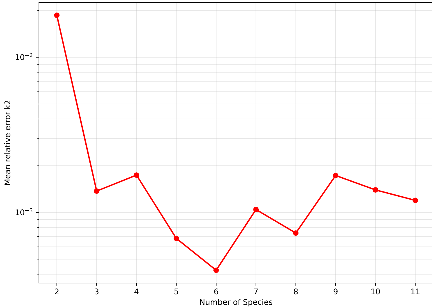
50, 50 — Mean relative error k2 vs number of species
